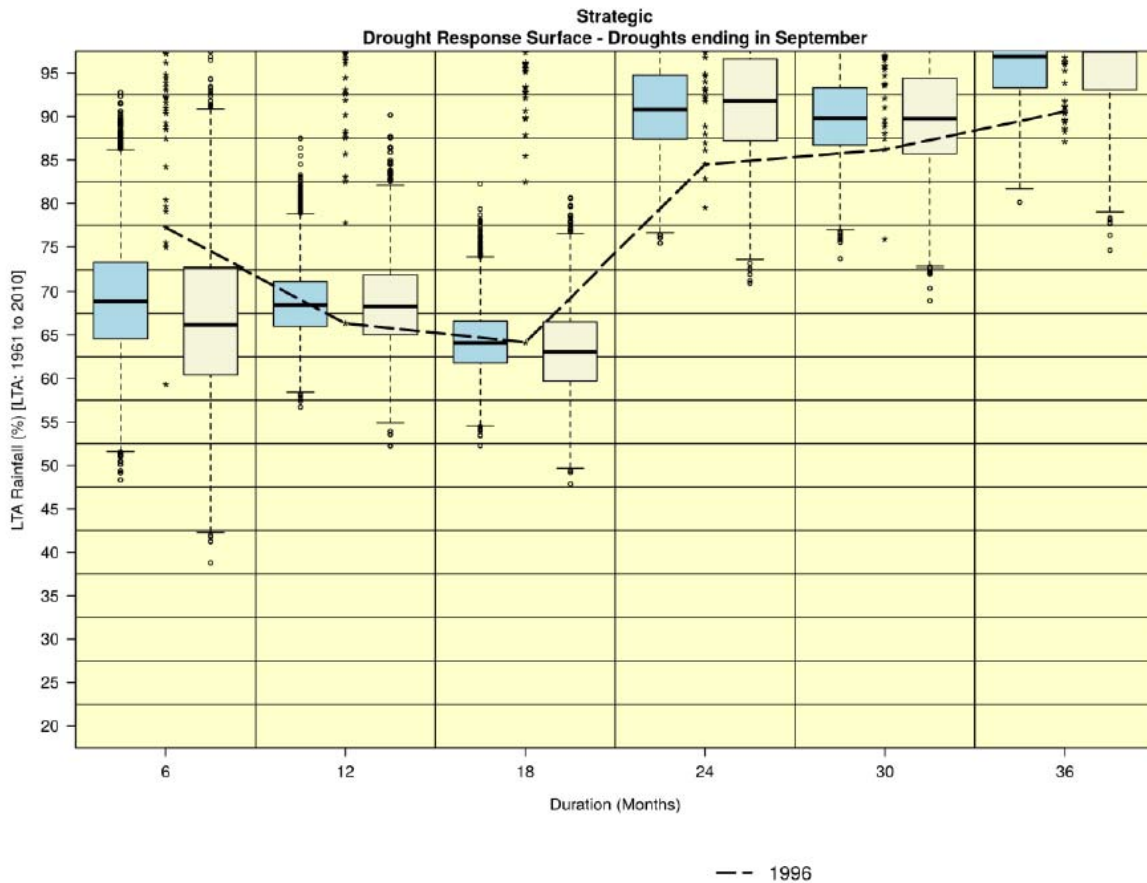
Figure 19 Drought Response Surface showing rainfall percentages of LTA (1961 to 2010) to September 1996 for selected durations (dashed line) and the impact of UKCP09 (blue box plots) and UKCP18 Probabilistic Projections (grey box plots) under a medium emission scenario (2070-2099 relative to a 1961-1990 baseline) on these values for 1995 to 1996. Black stars are rainfall percentages for different years (to September) in the historical record from 1961 to 2018.
