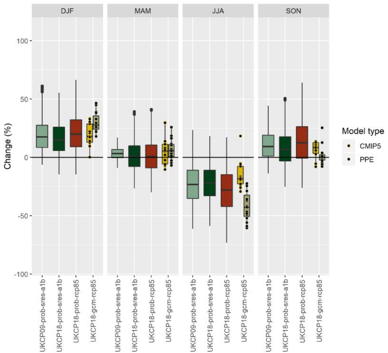
Figure 14 Change in seasonal rainfall for the UKCP18 North-West river basin. Changes are for the 2070-2099 future period relative to a 1961-1990 baseline, as used for WRMP19. Model type CMIP5 and PPE are types of global climate models. Source: Met Office 2019, United Utilities Water WRMP19
