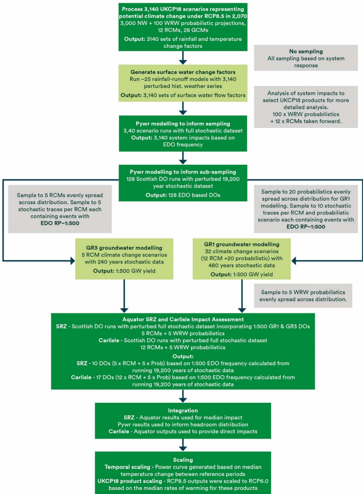
Figure 25 Summary of modelling workflow for assessing climate change
