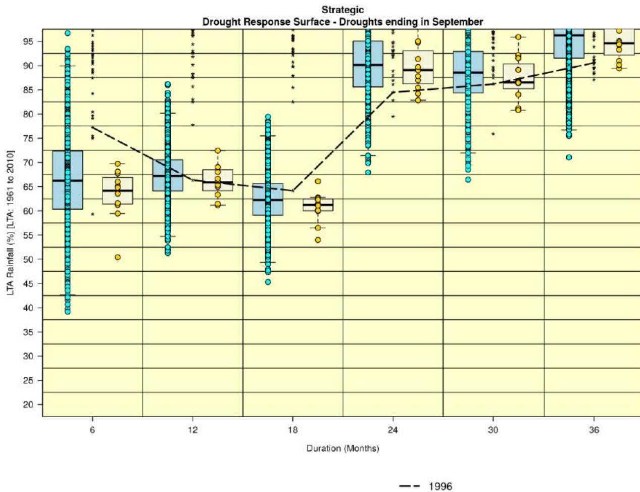
Figure 20 Drought Response Surface showing rainfall percentages of LTA (1961 to 2010) to September 1996 for selected durations (dashed line) and the impact of UKCP18 Probabilistic (blue box plots) and UKCP18 Regional Projections (grey box plots) under RCP 8.5 emissions scenario (2060-2079 relative to a 1981-2000 baseline) on these values for 1995 to 1996. Blue dots and yellow dots indicate specific scenarios. Black stars are rainfall percentages for different years (to September) in the historical record from 1961 to 2018.
