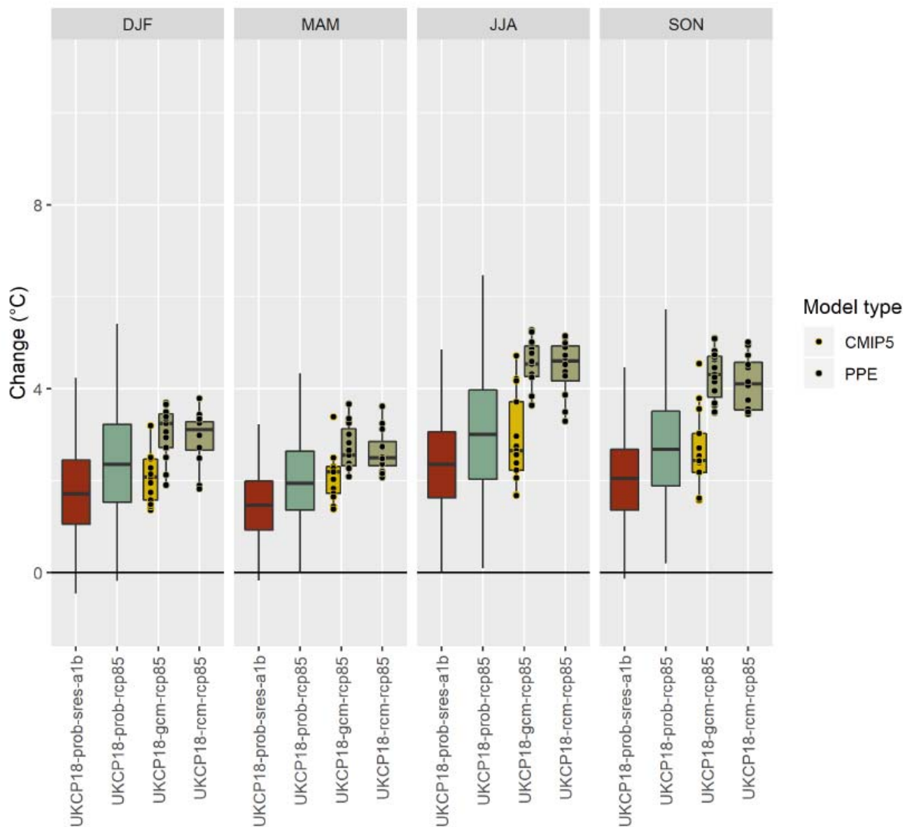
Figure 15 Changes in seasonal temperature for the UKCP18 North-West river basin. Changes are for the 2060-2079 future period relative to a 1981-2000 baseline. Model type CMIP5 and PPE are types of global climate models. Source: Met Office 2019, United Utilities Water WRMP19
