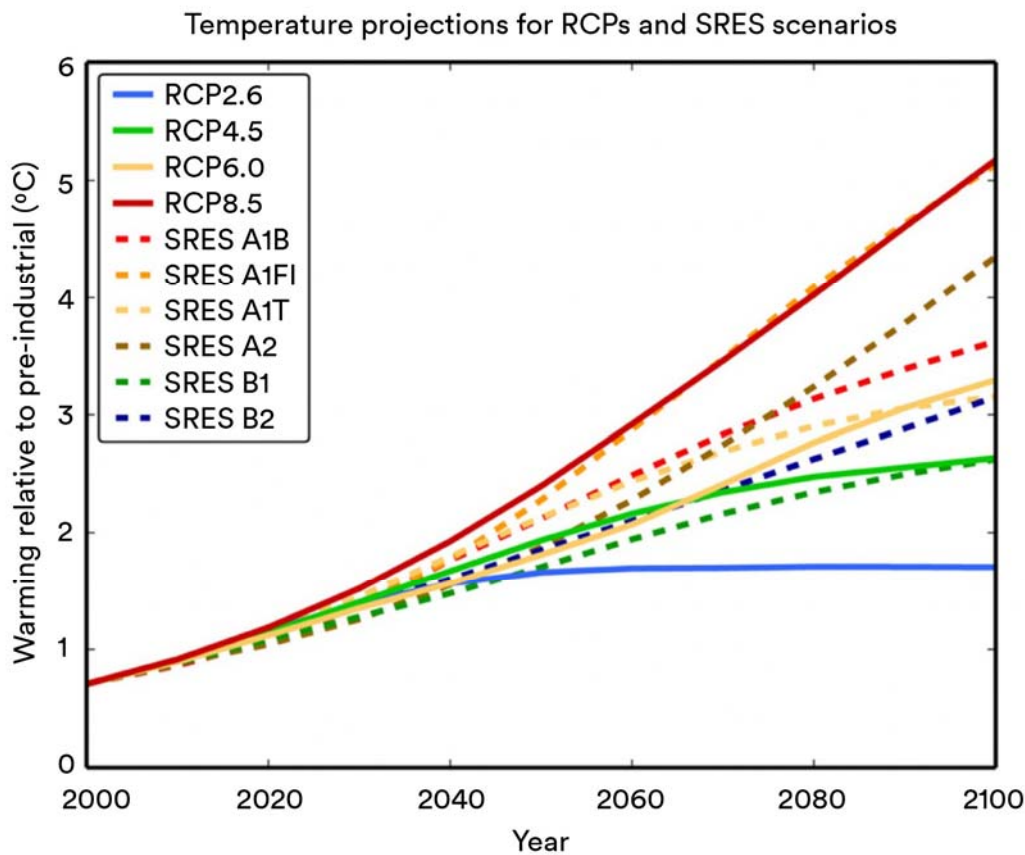
Figure 13 Global mean temperature projections from a climate model (called MAGICC6) relative to a pre-industrial average (1850-1900) for RCP2.6 (blue), RCP 4.5 (green), RCP 6.0 (yellow), and RCP 8.5 (red) and the older SRES scenarios (dashed coloured lines). Source: UK Met Office (2018)
