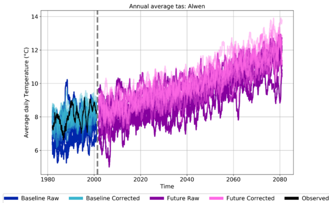
Figure 22 Bias corrected time series for the Alwen basin, highlighting underlying errors in the raw data, which is too cool for the baseline period
