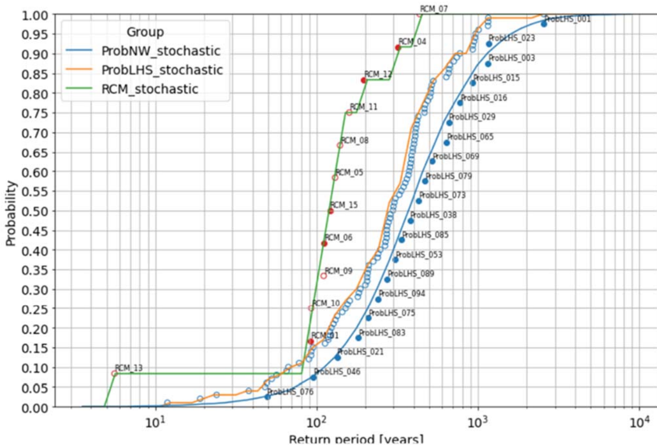
Figure 23 Distribution of EDO return period for all climate scenarios, simulated at a demand of 1800 MI/d. ProbLHS_stochastic refers to the 100 selected WRW factors for E&W, the solid blue circles show the ProbLHS scenarios once mapped to the distribution of the 3000 ProbNW scenarios
