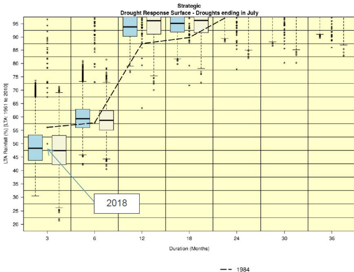
Figure 17 Drought Response Surface showing rainfall percentages of LTA (1961-2010) to July 1984 for selected durations (dashed line) and the impact of UKCP09 (blue box plots) and UKCP18 Probabilistic Projections (grey box plots) under a medium emissions scenario (2070-2099 relative to a 1961-1990 baseline) on these values for 1984. Black stars are rainfall percentages for different years (to July) in the historical record from 1961-2018.
