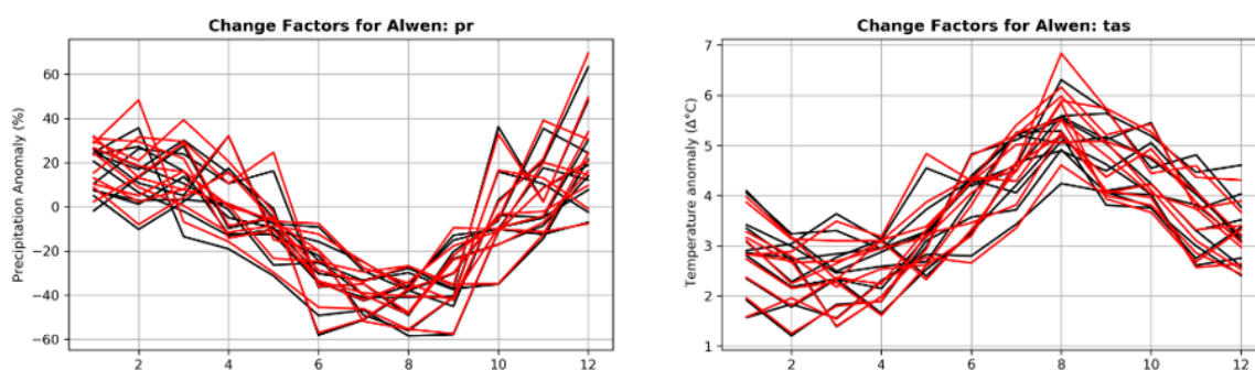
Figure 21 Comparison of bias corrected monthly change factors (red) and raw factors (black) for the Alwen basin for precipitation (pr) and average temperature (tas)
