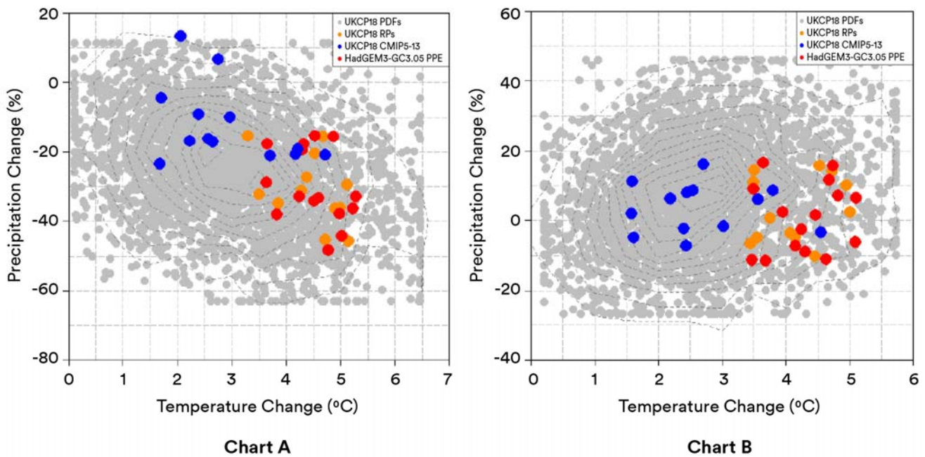
Figure 16 Changes in summer (5b autumn) temperature and precipitation for the UKCP18 North-West river basin. Changes are for the 2060-2079 future period relative to a 1981-2000 baseline. Probabilistic Projections are shown by grey circles, Regional Projection are shown in orange circle, CMPI5-13 Global Projections are shown in blue circles, and the HadGEM3-GC3.05 Global Projections in red circles. Source: Met Office 2019
