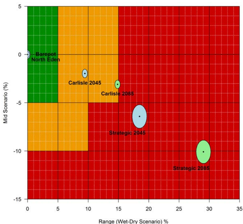
Figure 12 Climate change magnitude-sensitivity plot for all RZs for 2045 and 2085
