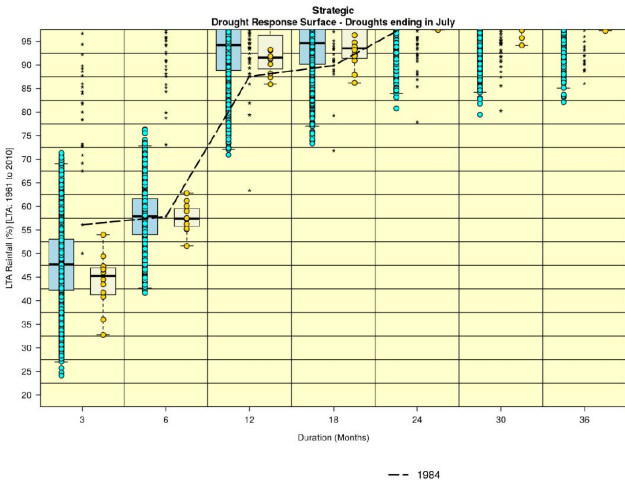
Figure 18 Drought Response Surface showing rainfall percentages of LTA (1961-2010) to July 1984 for selected durations (dashed line) and the impact of UKCP18 Probabilistic Projections (blue box plots) and UKCP18 Regional Projections (grey box plots) under RCP 8.5 emission scenario (2060-2079 relative to a 1981-2000 baseline) on these values for 1984. Blue dots and yellow dots indicate specific scenarios. Black stars are rainfall percentages for different years (to July) in the historical record from 1961 to 2018.
